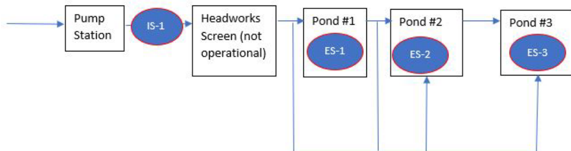
Figure 1. Process Flow Diagram with Sampling Locations
